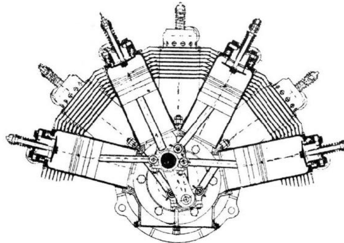
7 cylinder.
