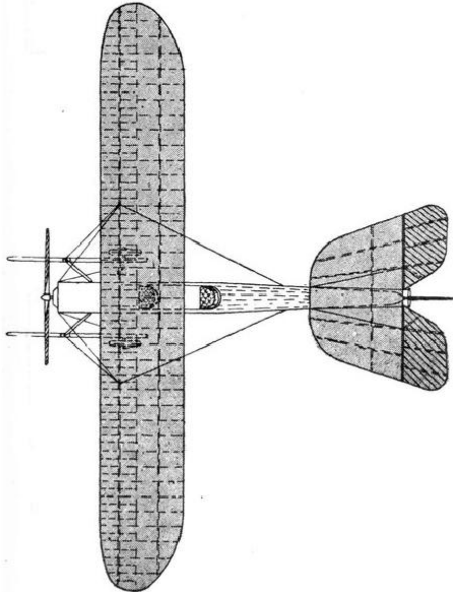
B.E. type. R.A.F. Uniform Aeroplane Scale
