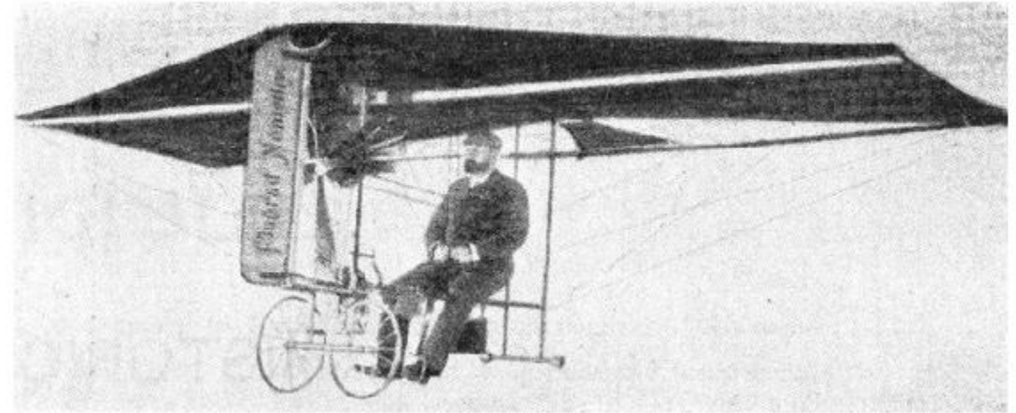
SOLTAU (1910). An ornithopter based on the earlier ideas of Adhemar de la Hault (see Belgium).
