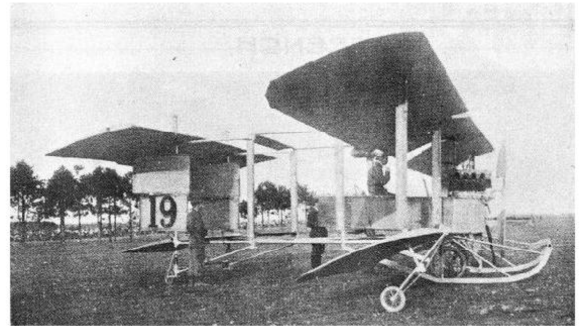
BREGUET IV (1910). On its appearance, this machine was generally laughed at and nicknamed the "Coffee Pot," till in Aug., 1910, it made a world's record by carrying six, and later proved itself superior in stability to anything then existing.
