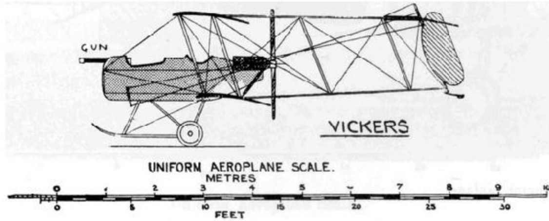
VICKERS. Uniform Aeroplane Scale
