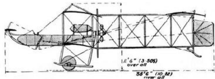
Short. S. 38 military.
