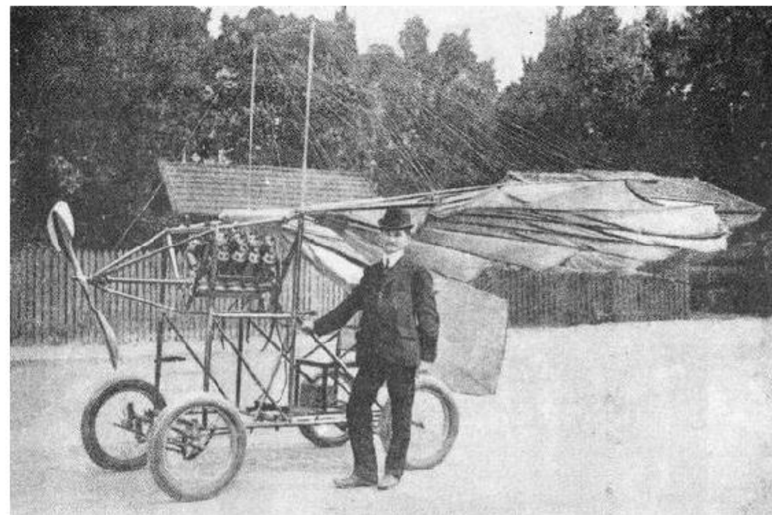
VUIA (1908). Earliest known machine with folding wings.
