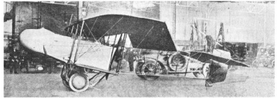
H. Farman. 1913 latest type military biplane.
