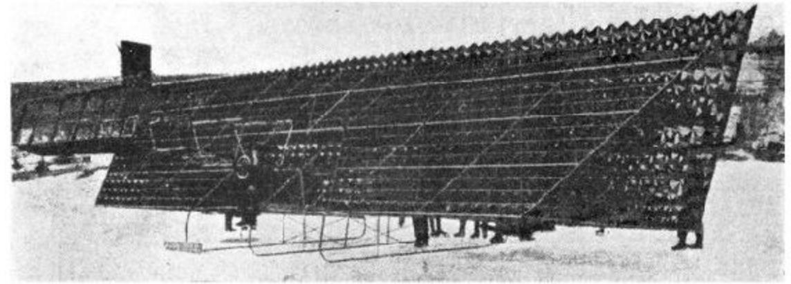
CYGNET II (1908). Designed by Dr. Graham Bell, of the Aeronautical Society of America. Bell (Canadian), Glen Curtiss (U.S.), Herring (U.S.), and Burgess (Canadian). It made short flights.
