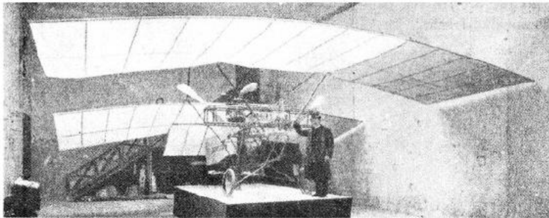
HIPSSICH (1908). Tandem mono. with one propeller before and another in rear of rear plane.
