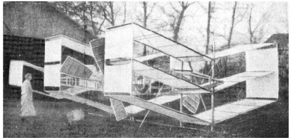
DUFAUX (1908-09). First Swiss machine.
