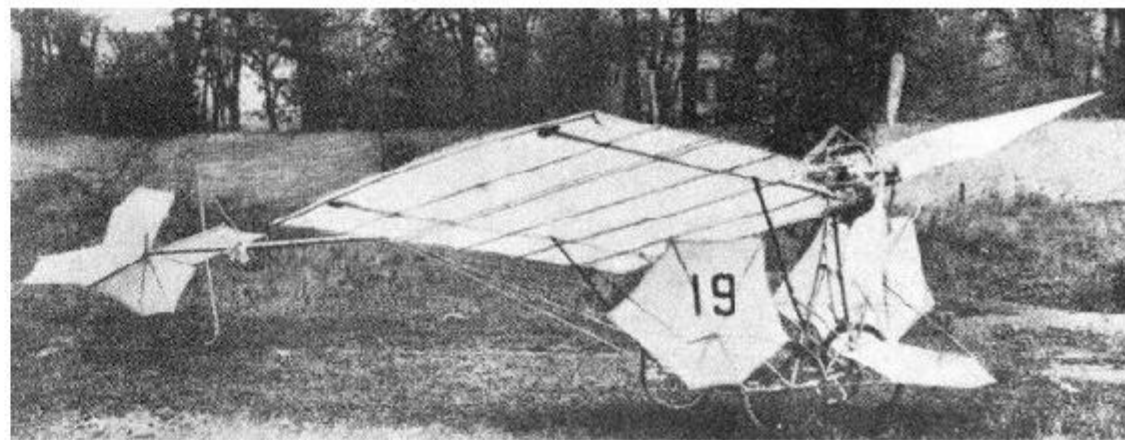
SANTOS-DUMONT XIX. This little machine, surface only 9 m 2 . made an extraordinary sensation in France in 1909. It flew at the then incredible speed of 65 m.p.h. (100 k.p.h.) Santos-Dumont presented all rights to the world soon afterwards, and a large number were built before it was realised that only an extremely light weight pilot could fly in one. Few of the copies ever left the ground.
