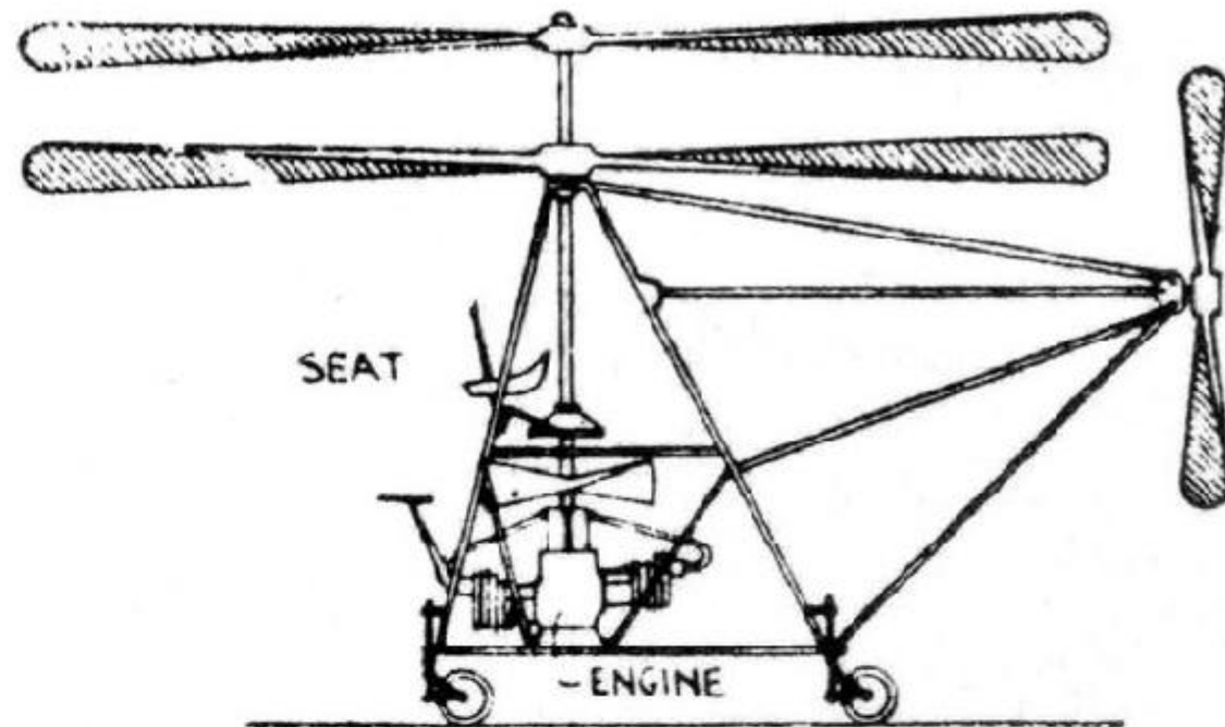
VUITTON-HUBER (1908). Early helicopter.
